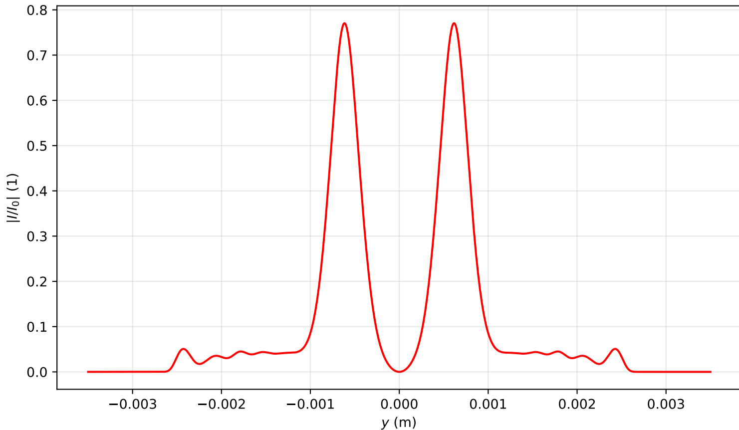
Intensity profile I(x=0, y, z=2.468)/I_0 , P_{in}=6.0P_{cr} , artificial time
